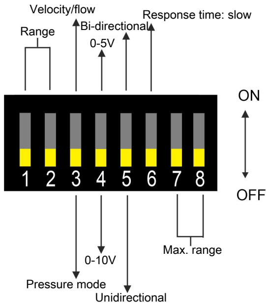
Figure 4: Setting dipswitches.
